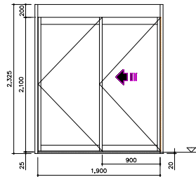
Elevation SCALE 1/30
